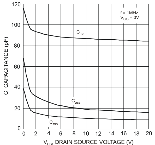
Fig. 12 Capacitance Variation
